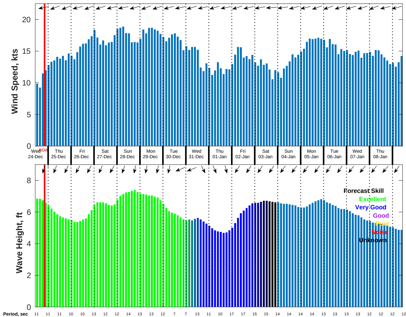
Wind & Wave Forecast for NDBC 52213 from 23-Dec-2025 11:00:00 to 08-Jan-2026 11:00:00
