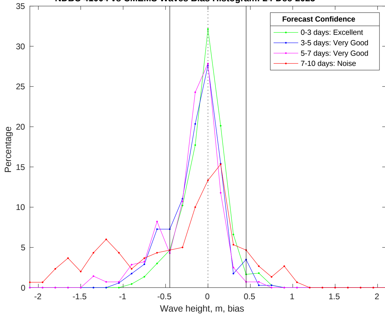
NDBC 41004 vs CMEMS Waves Bias Histogram: 24-Dec-2025
