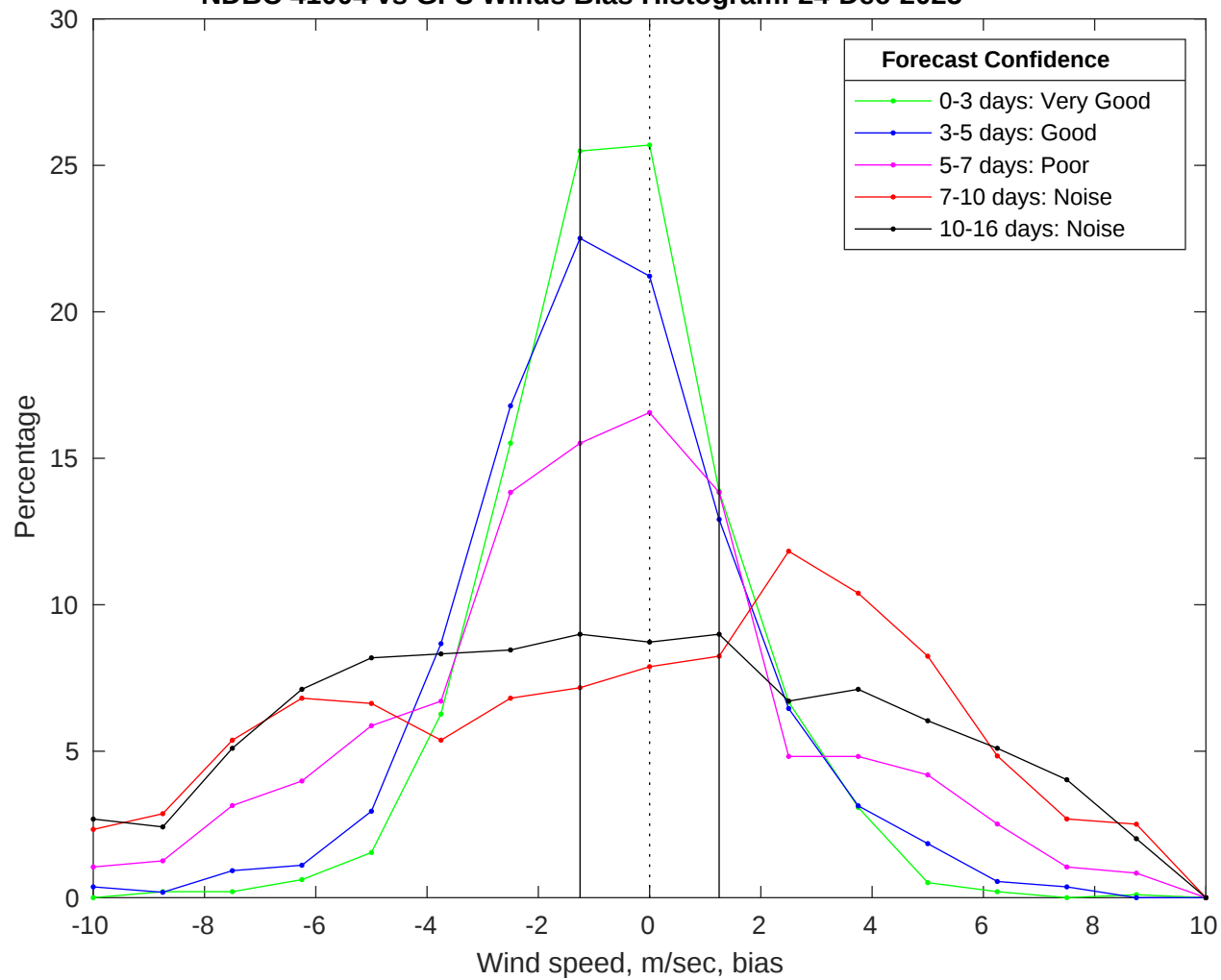
NDBC 41004 vs GFS Winds Bias Histogram: 24-Dec-2025
