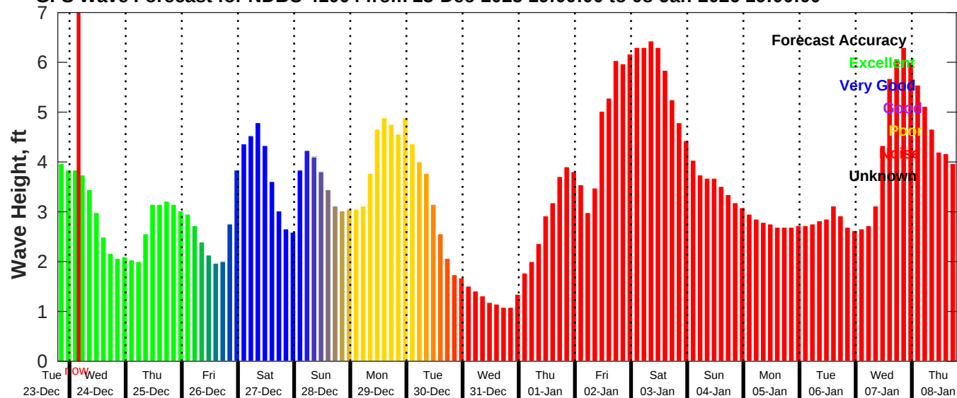
GFS Wave Forecast for NDBC 41004 from 23-Dec-2025 19:00:00 to 08-Jan-2026 19:00:00
