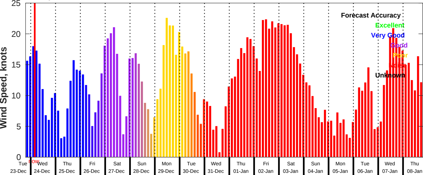
GFS Wind Speed Forecast for NDBC 41004 from 23-Dec-2025 19:00:00 to 08-Jan-2026 19:00:00
