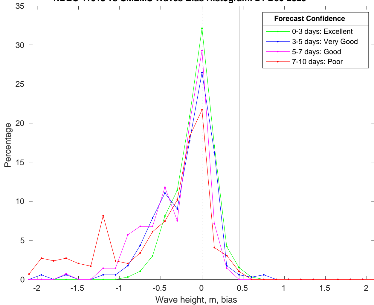
NDBC 41013 vs CMEMS Waves Bias Histogram: 24-Dec-2025
