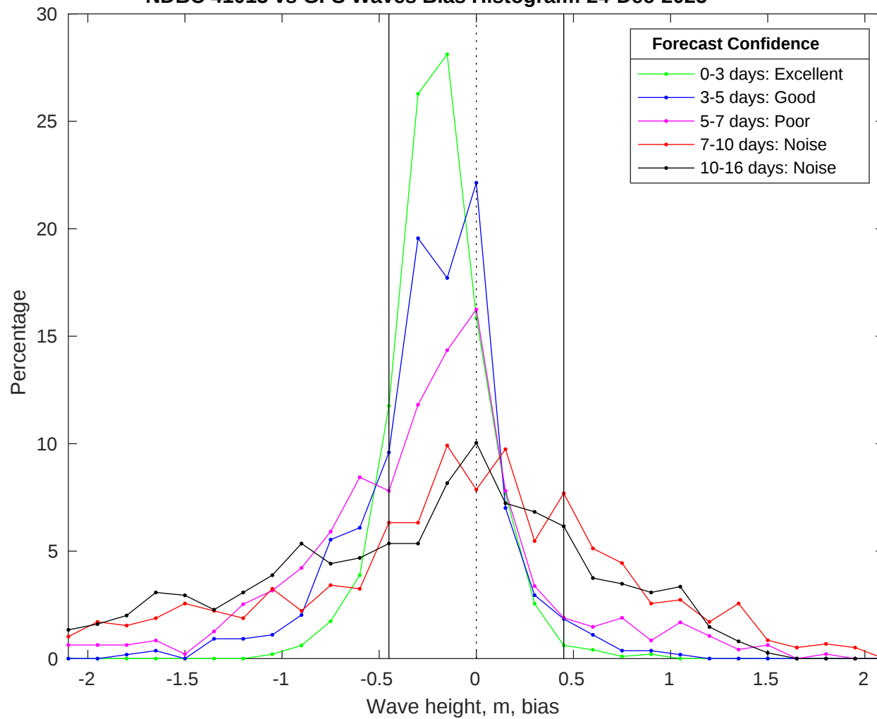
NDBC 41013 vs GFS Waves Bias Histogram: 24-Dec-2025
