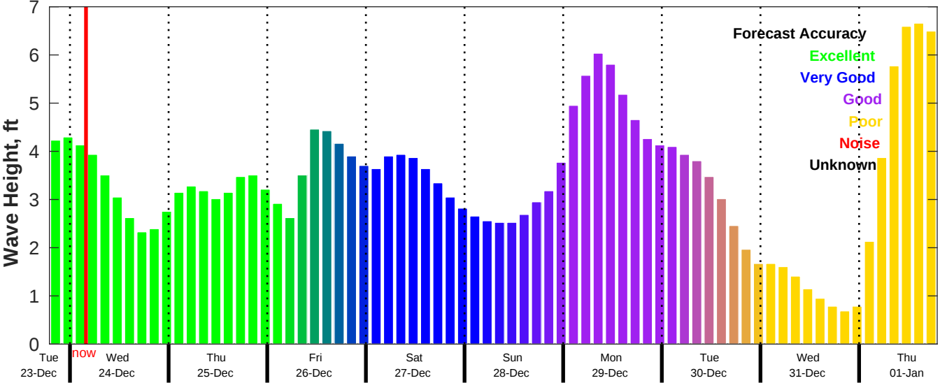
CMEMS Wave Forecast for NDBC 41013 from 23-Dec-2025 19:00:00 to 01-Jan-2026 19:00:00
