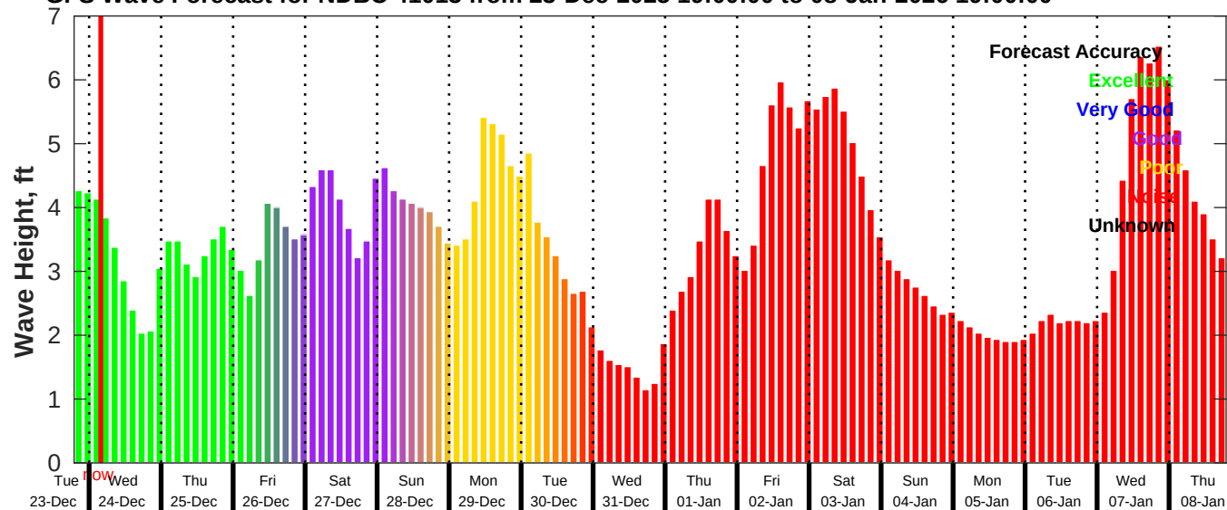
GFS Wave Forecast for NDBC 41013 from 23-Dec-2025 19:00:00 to 08-Jan-2026 19:00:00
