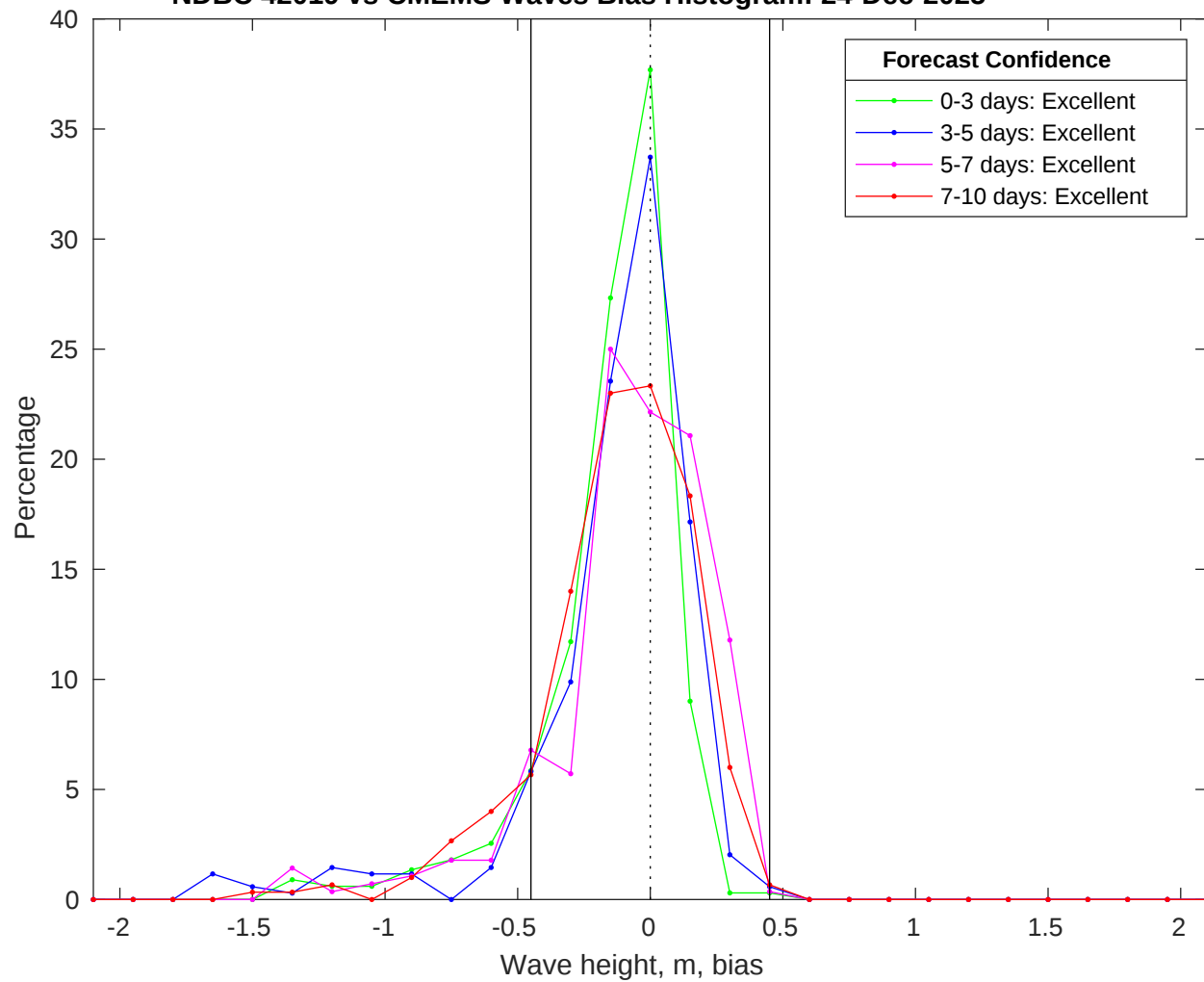
NDBC 42019 vs CMEMS Waves Bias Histogram: 24-Dec-2025
