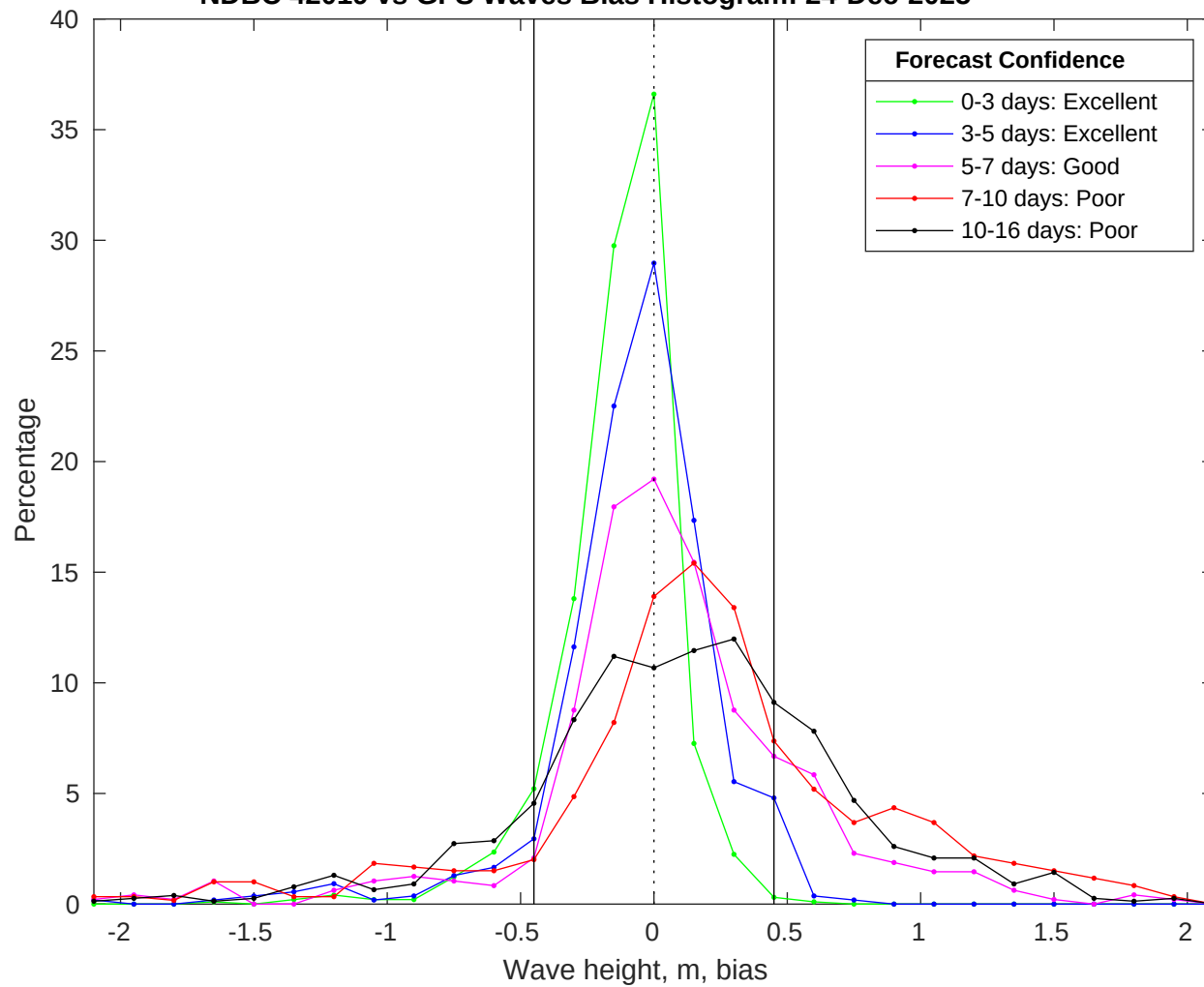
NDBC 42019 vs GFS Waves Bias Histogram: 24-Dec-2025
