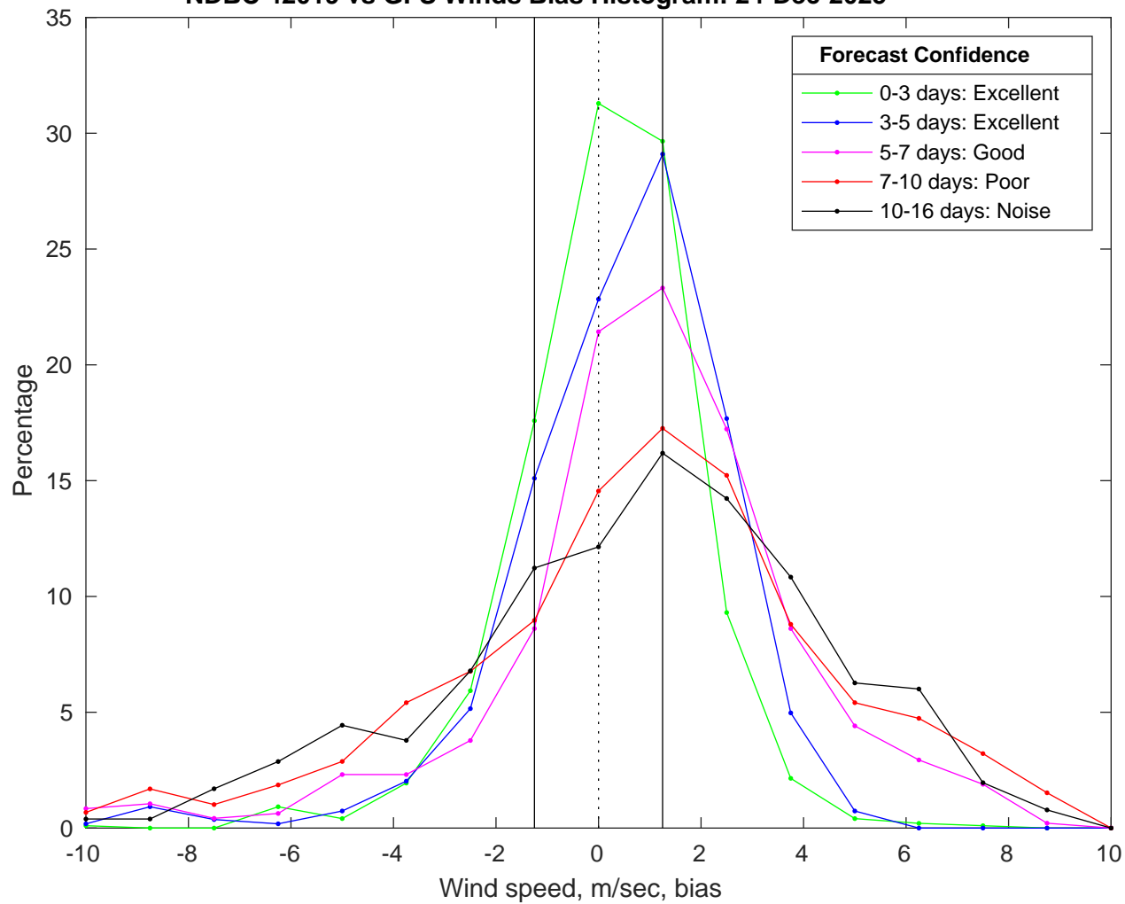
NDBC 42019 vs GFS Winds Bias Histogram: 24-Dec-2025
