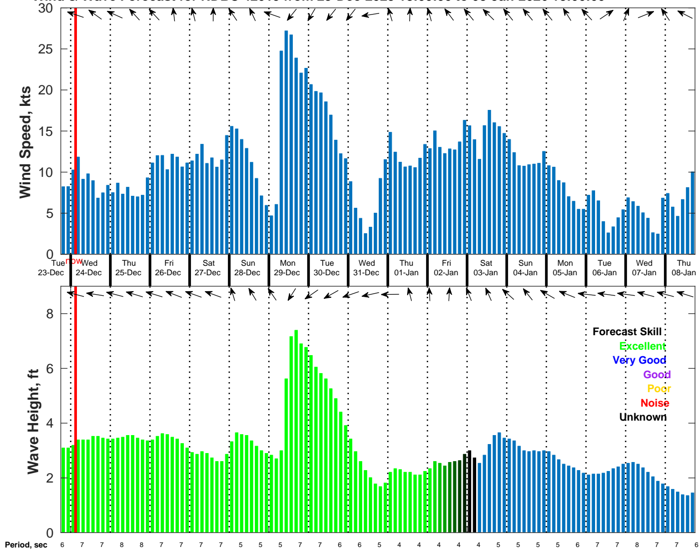
Wind & Wave Forecast for NDBC 42019 from 23-Dec-2025 18:00:00 to 08-Jan-2026 18:00:00
