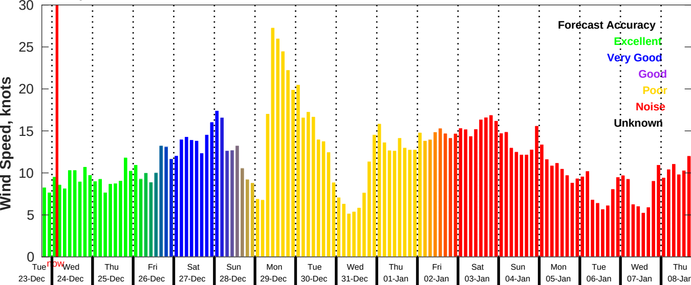
GFS Wind Speed Forecast for NDBC 42020 from 23-Dec-2025 18:00:00 to 08-Jan-2026 18:00:00
