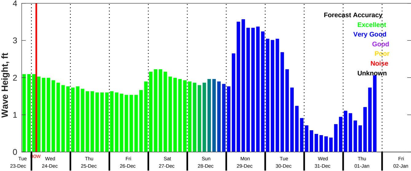
CMEMS Wave Forecast for NDBC 42035 from 23-Dec-2025 18:00:00 to 02-Jan-2026 18:00:00
