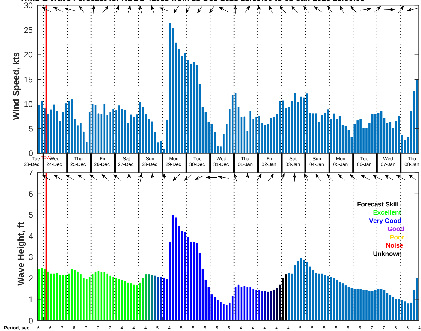
Wind & Wave Forecast for NDBC 42035 from 23-Dec-2025 18:00:00 to 08-Jan-2026 18:00:00
