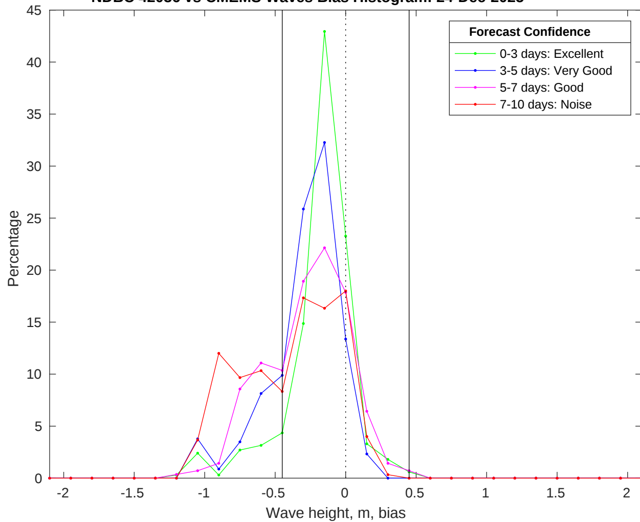
NDBC 42036 vs CMEMS Waves Bias Histogram: 24-Dec-2025
