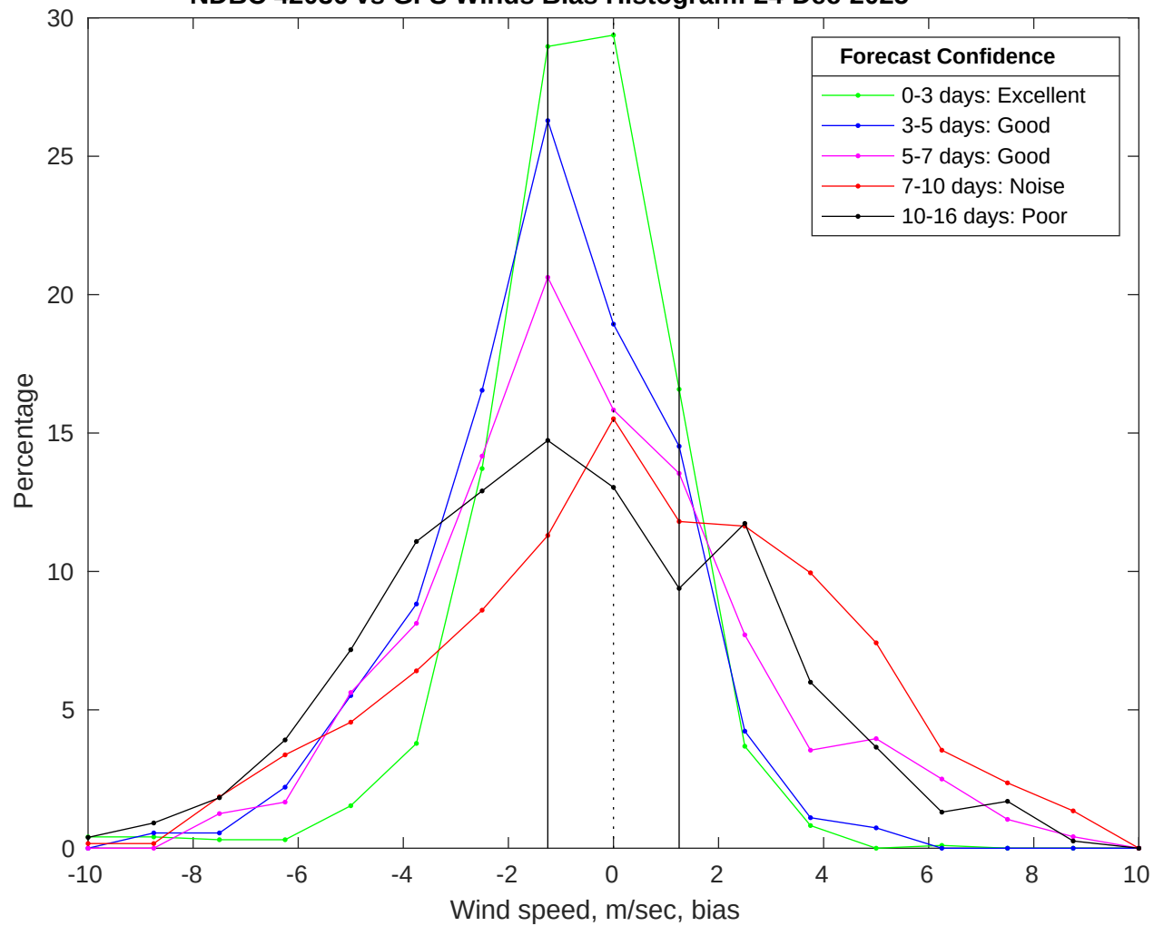
NDBC 42036 vs GFS Winds Bias Histogram: 24-Dec-2025
