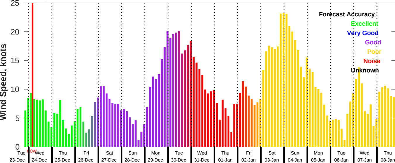
GFS Wind Speed Forecast for NDBC 42036 from 23-Dec-2025 19:00:00 to 08-Jan-2026 19:00:00
