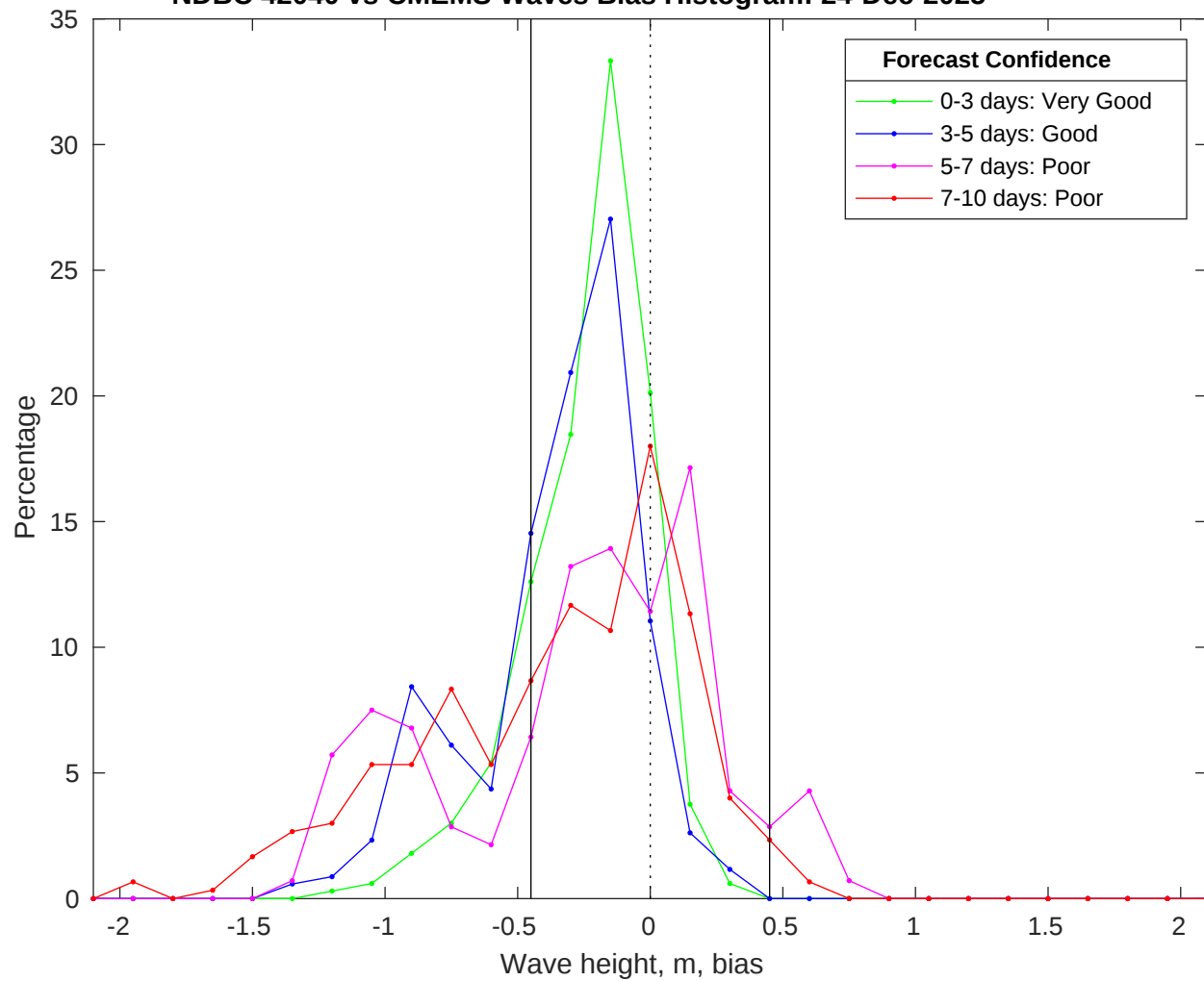
NDBC 42040 vs CMEMS Waves Bias Histogram: 24-Dec-2025
