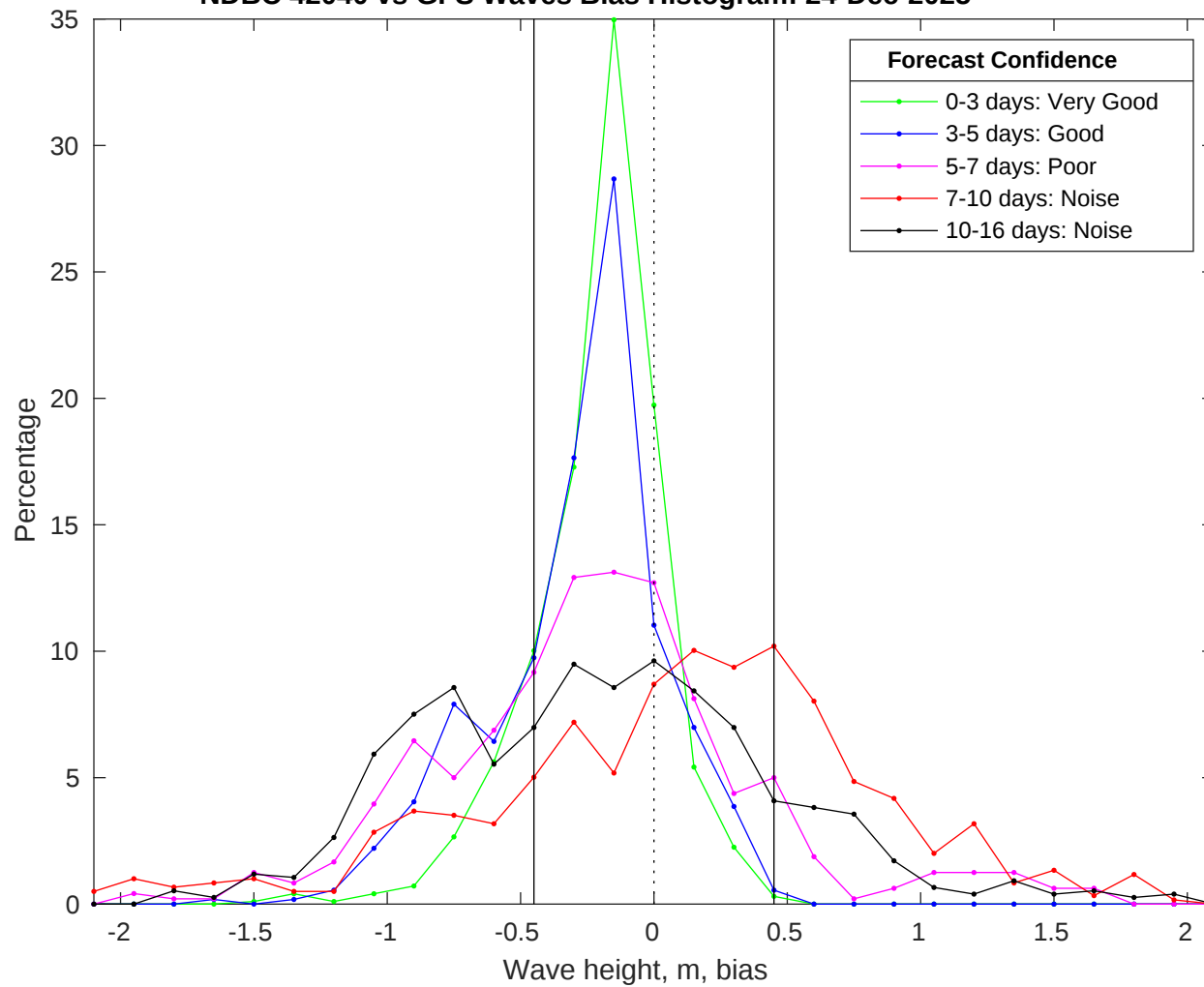
NDBC 42040 vs GFS Waves Bias Histogram: 24-Dec-2025
