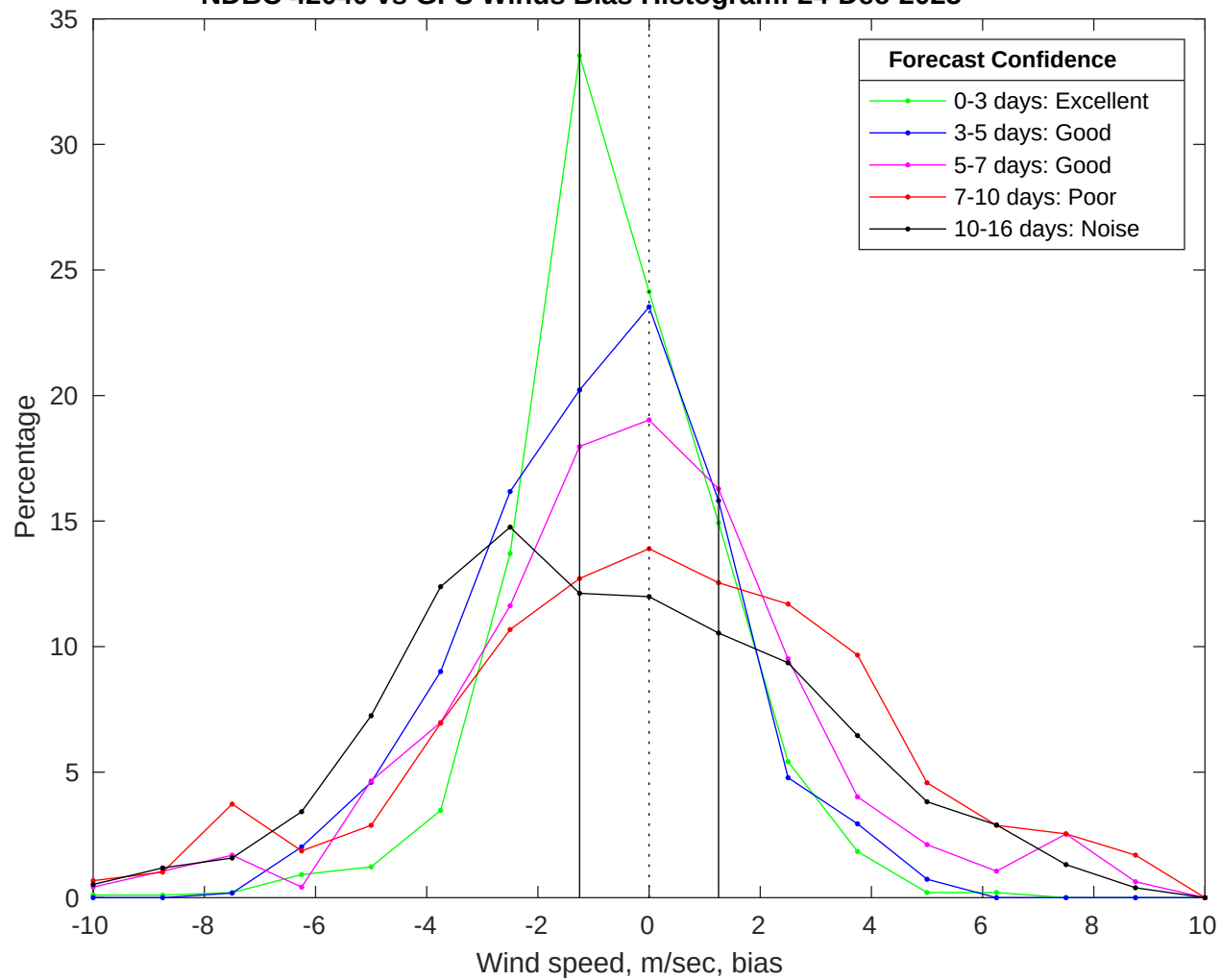
NDBC 42040 vs GFS Winds Bias Histogram: 24-Dec-2025
