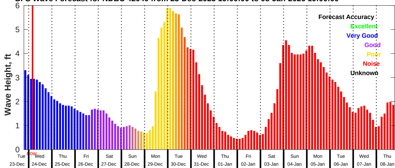
GFS Wave Forecast for NDBC 42040 from 23-Dec-2025 19:00:00 to 08-Jan-2026 19:00:00
