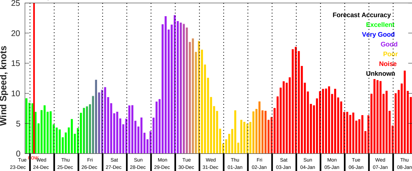
GFS Wind Speed Forecast for NDBC 42040 from 23-Dec-2025 19:00:00 to 08-Jan-2026 19:00:00
