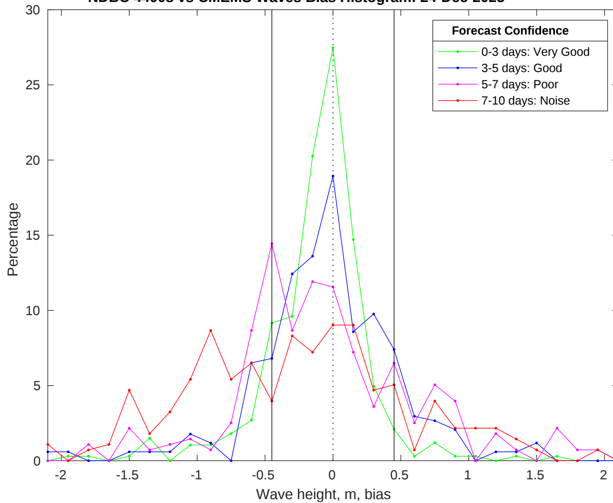
NDBC 44008 vs CMEMS Waves Bias Histogram: 24-Dec-2025
