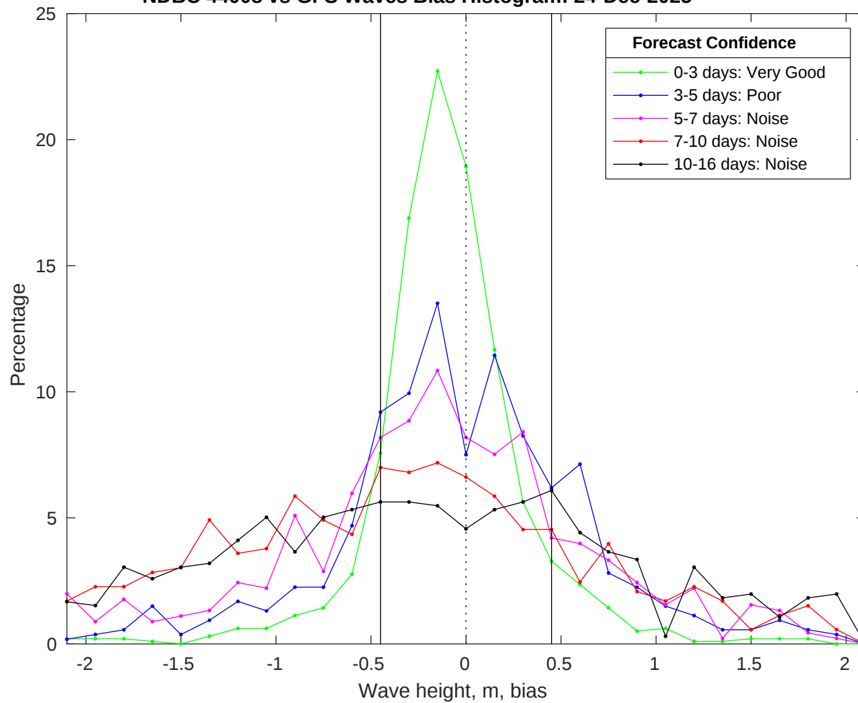
NDBC 44008 vs GFS Waves Bias Histogram: 24-Dec-2025
