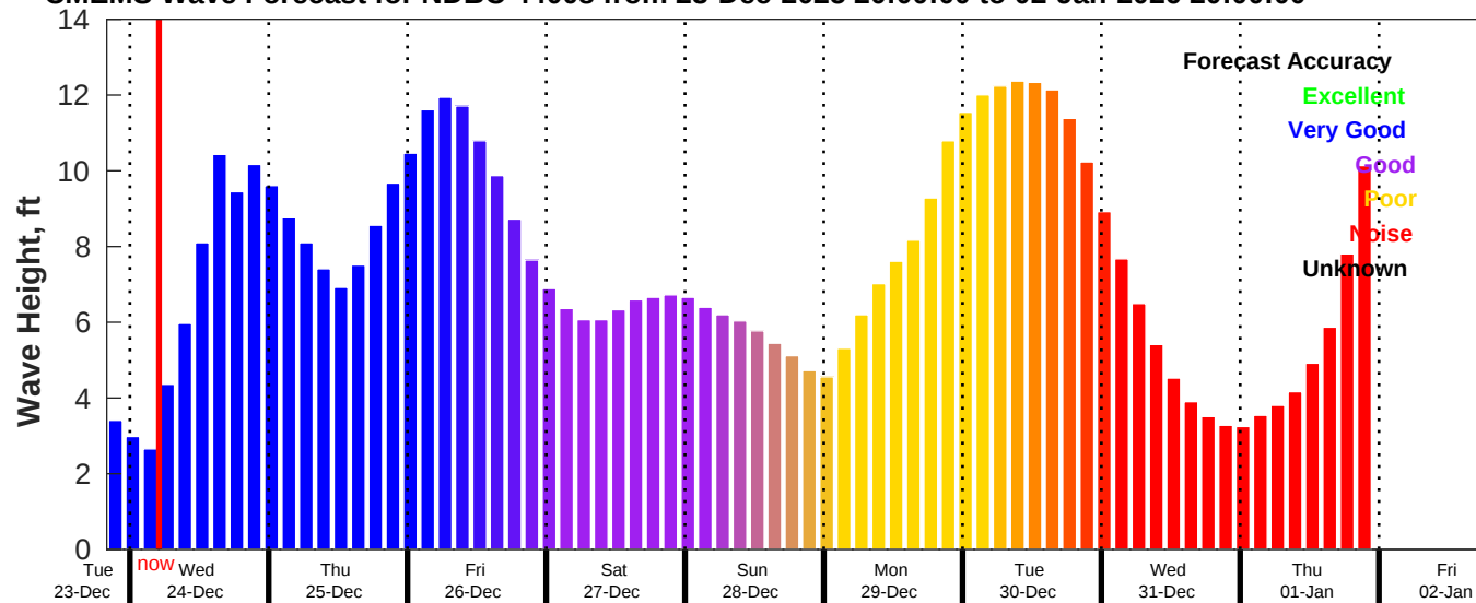
CMEMS Wave Forecast for NDBC 44008 from 23-Dec-2025 20:00:00 to 02-Jan-2026 20:00:00
