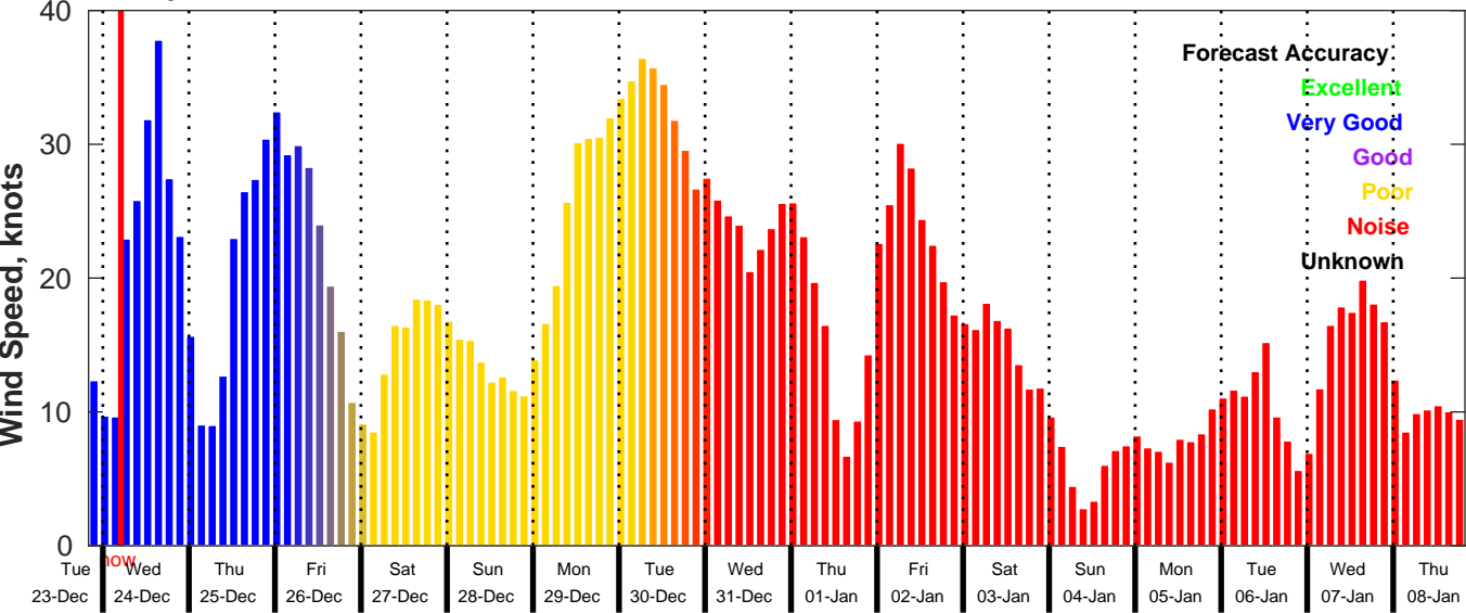
GFS Wind Speed Forecast for NDBC 44008 from 23-Dec-2025 20:00:00 to 08-Jan-2026 20:00:00
