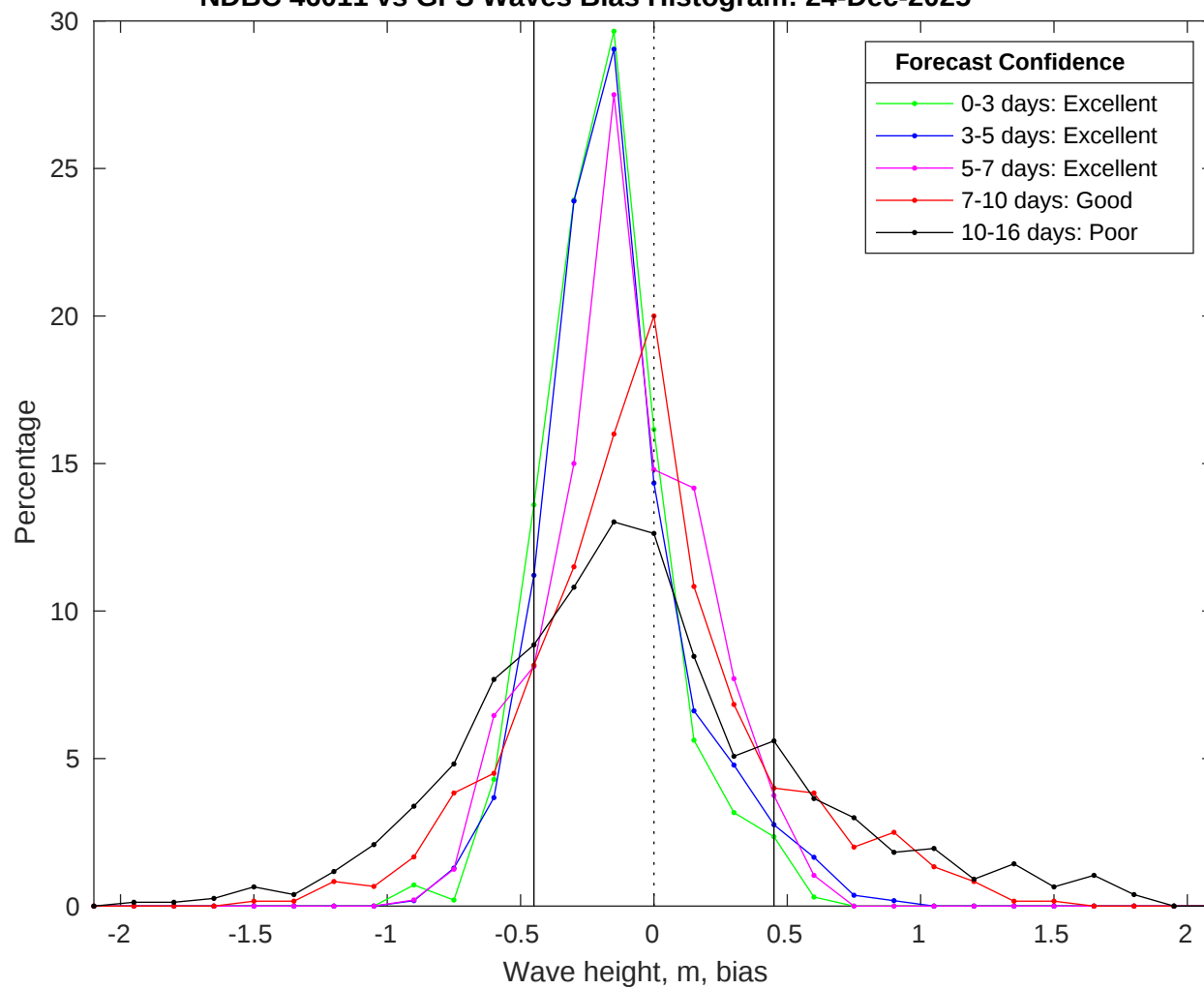
NDBC 46011 vs GFS Waves Bias Histogram: 24-Dec-2025
