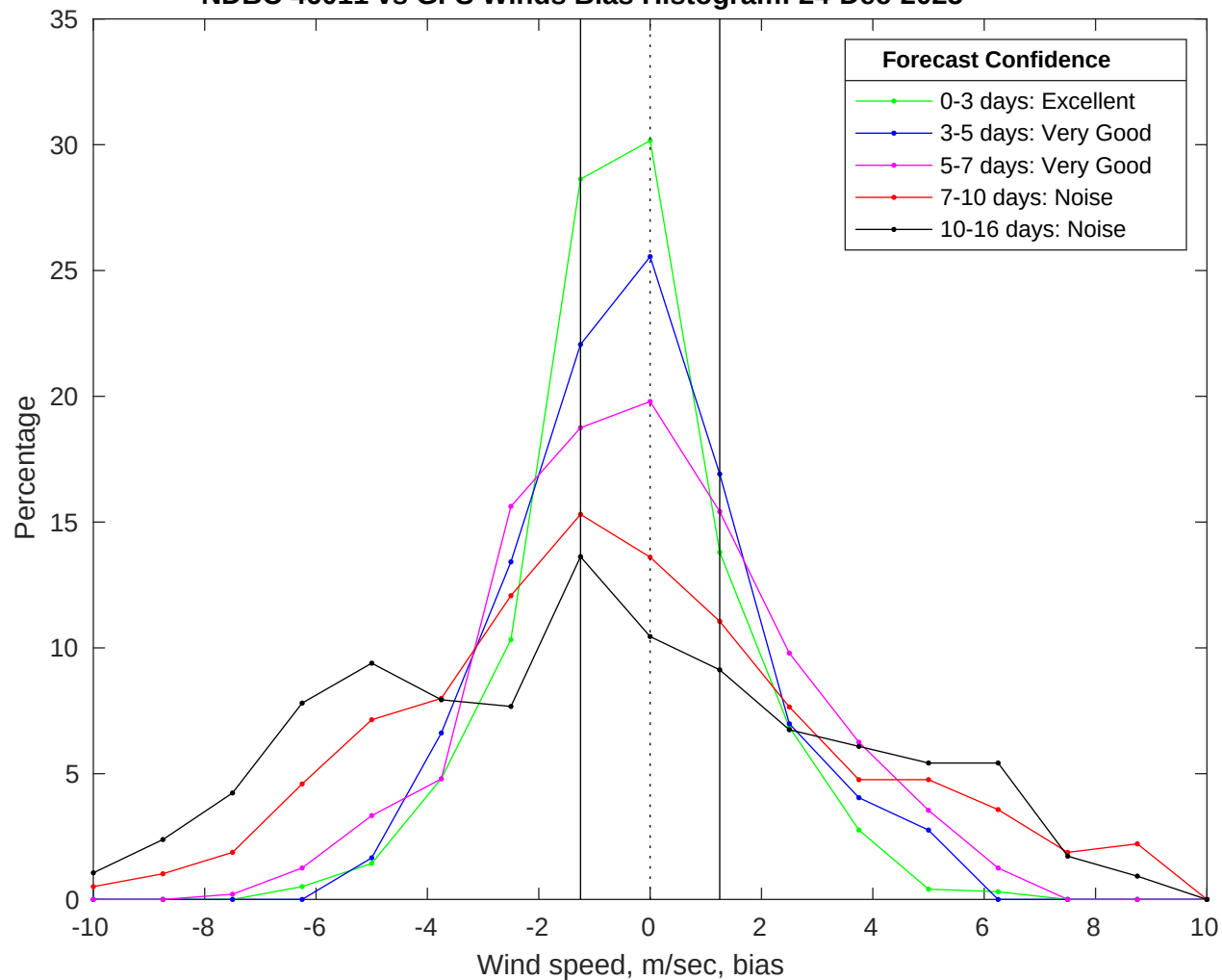
NDBC 46011 vs GFS Winds Bias Histogram: 24-Dec-2025
