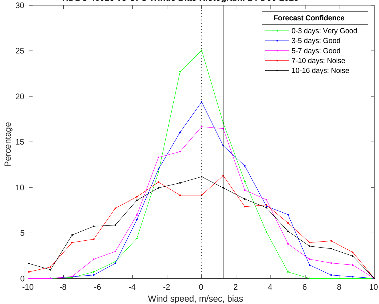
NDBC 46028 vs GFS Winds Bias Histogram: 24-Dec-2025
