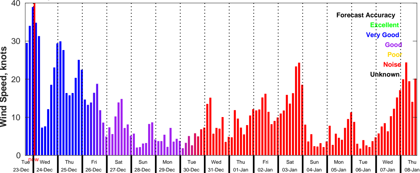
GFS Wind Speed Forecast for NDBC 46028 from 23-Dec-2025 16:00:00 to 08-Jan-2026 16:00:00
