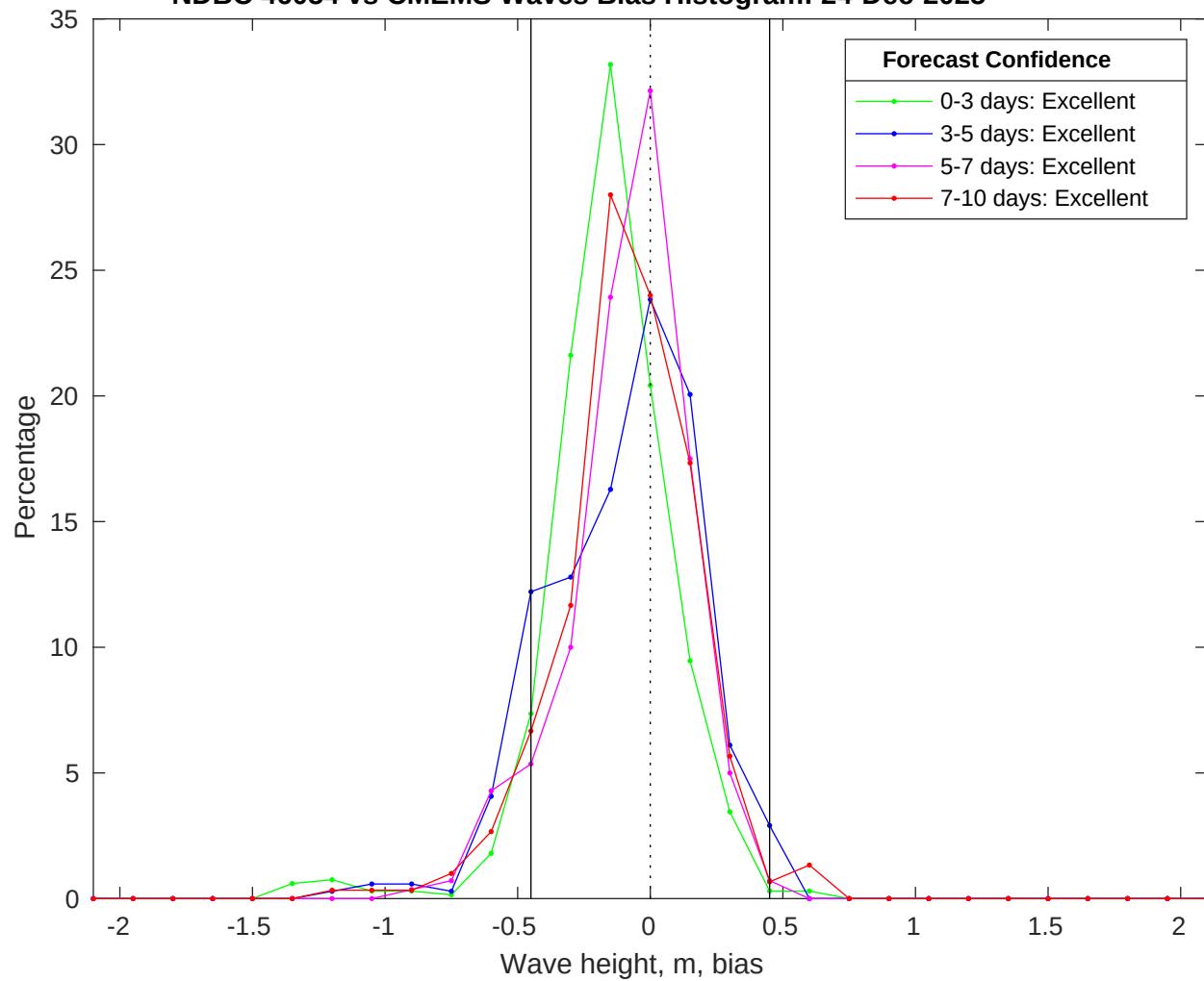
NDBC 46054 vs CMEMS Waves Bias Histogram: 24-Dec-2025
