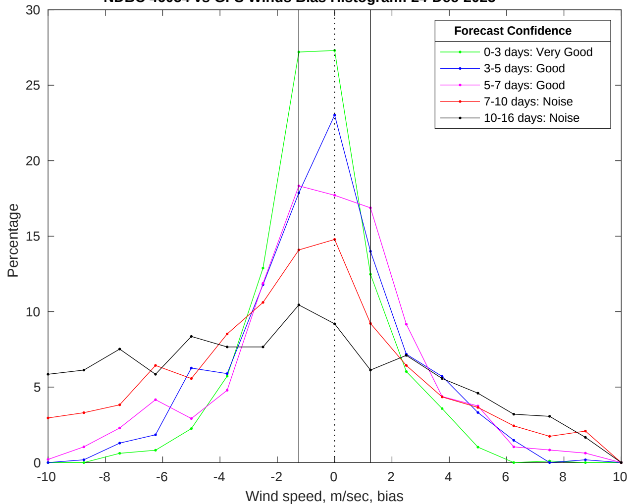
NDBC 46054 vs GFS Winds Bias Histogram: 24-Dec-2025
