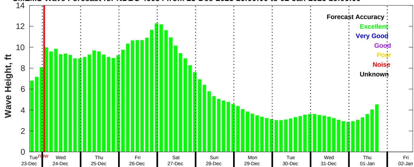
CMEMS Wave Forecast for NDBC 46054 from 23-Dec-2025 16:00:00 to 02-Jan-2026 16:00:00
