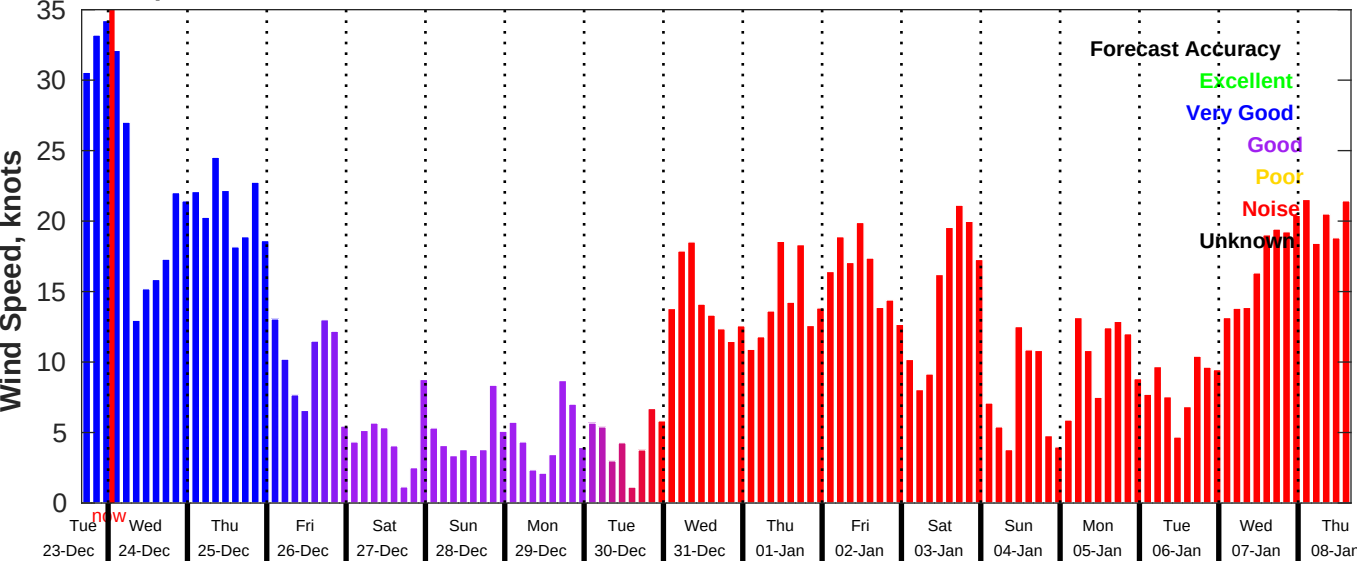
GFS Wind Speed Forecast for NDBC 46054 from 23-Dec-2025 16:00:00 to 08-Jan-2026 16:00:00
