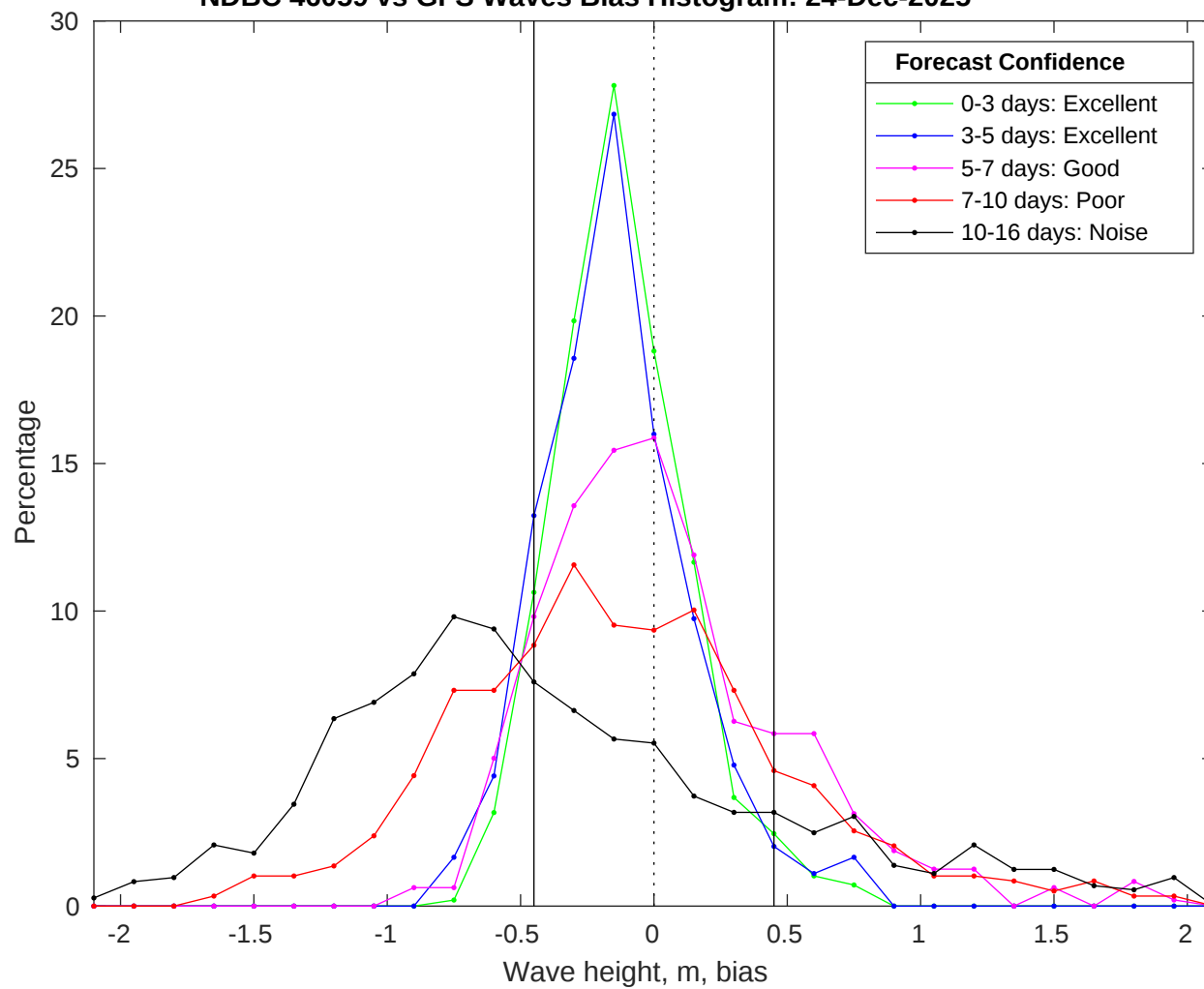
NDBC 46059 vs GFS Waves Bias Histogram: 24-Dec-2025
