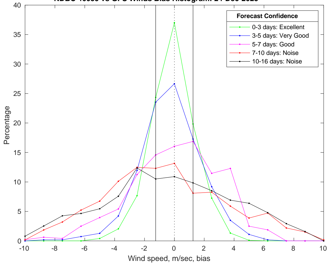
NDBC 46059 vs GFS Winds Bias Histogram: 24-Dec-2025
