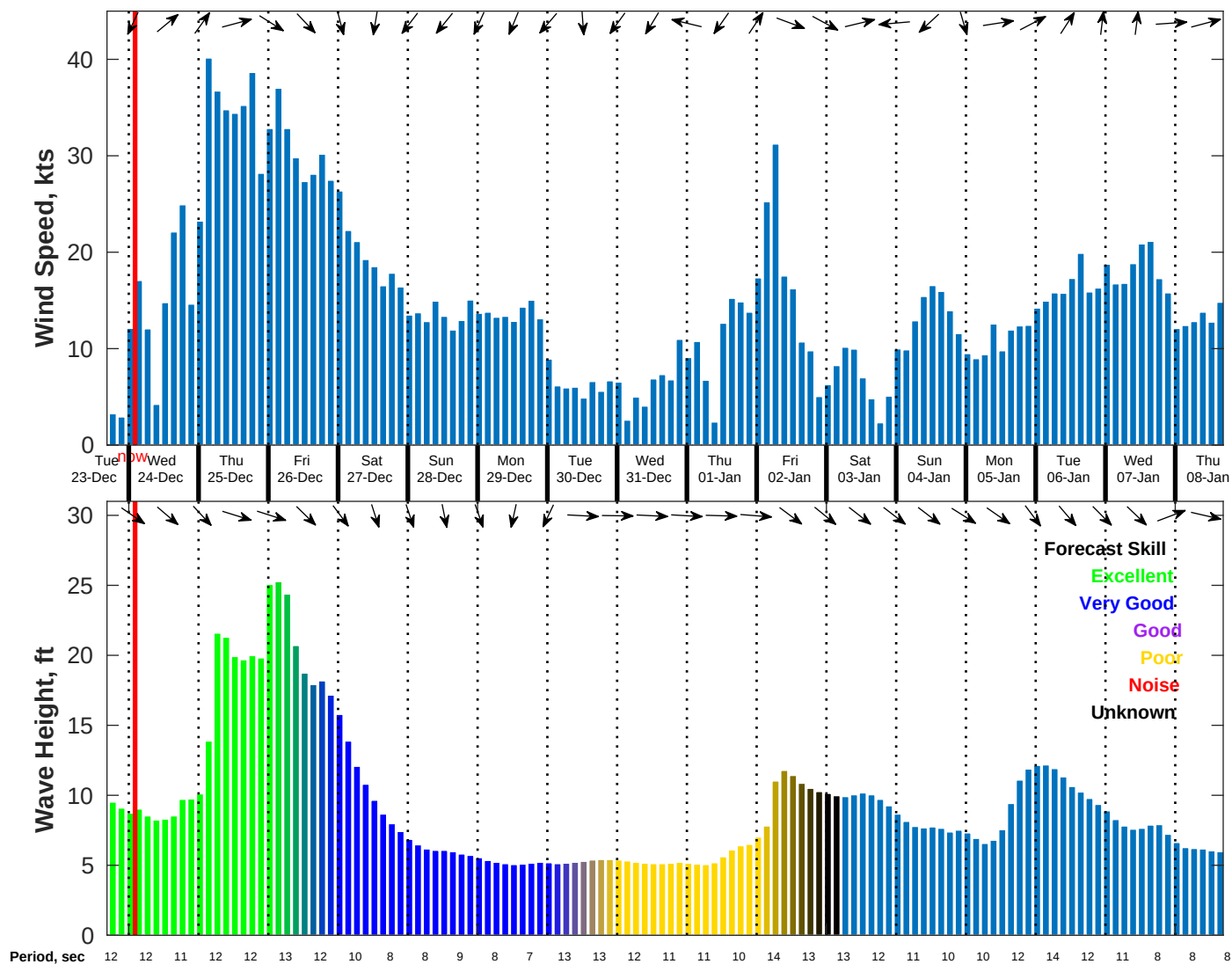
Wind & Wave Forecast for NDBC 46059 from 23-Dec-2025 17:00:00 to 08-Jan-2026 17:00:00
