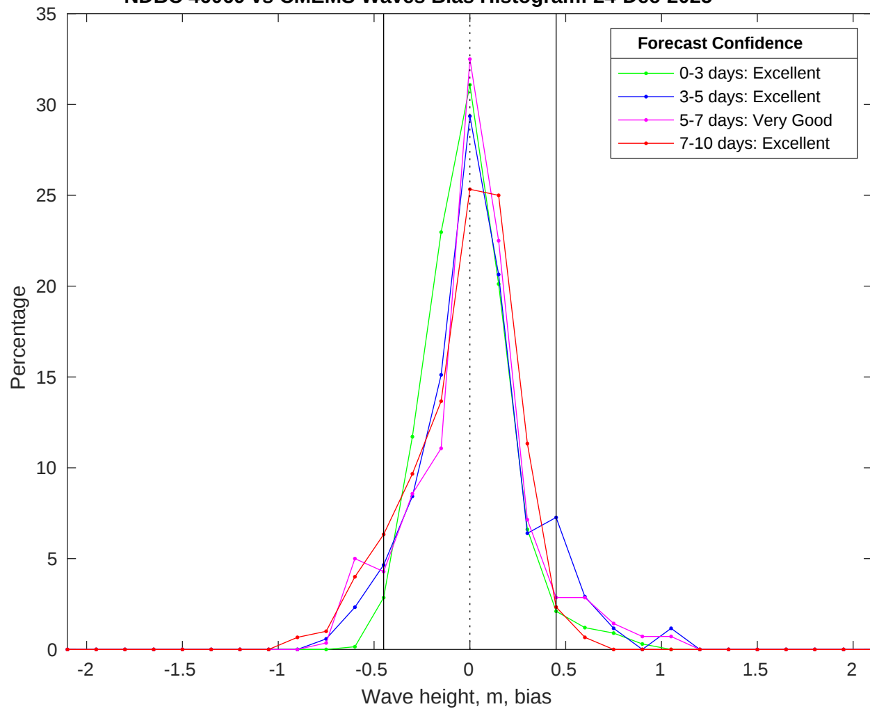
NDBC 46069 vs CMEMS Waves Bias Histogram: 24-Dec-2025
