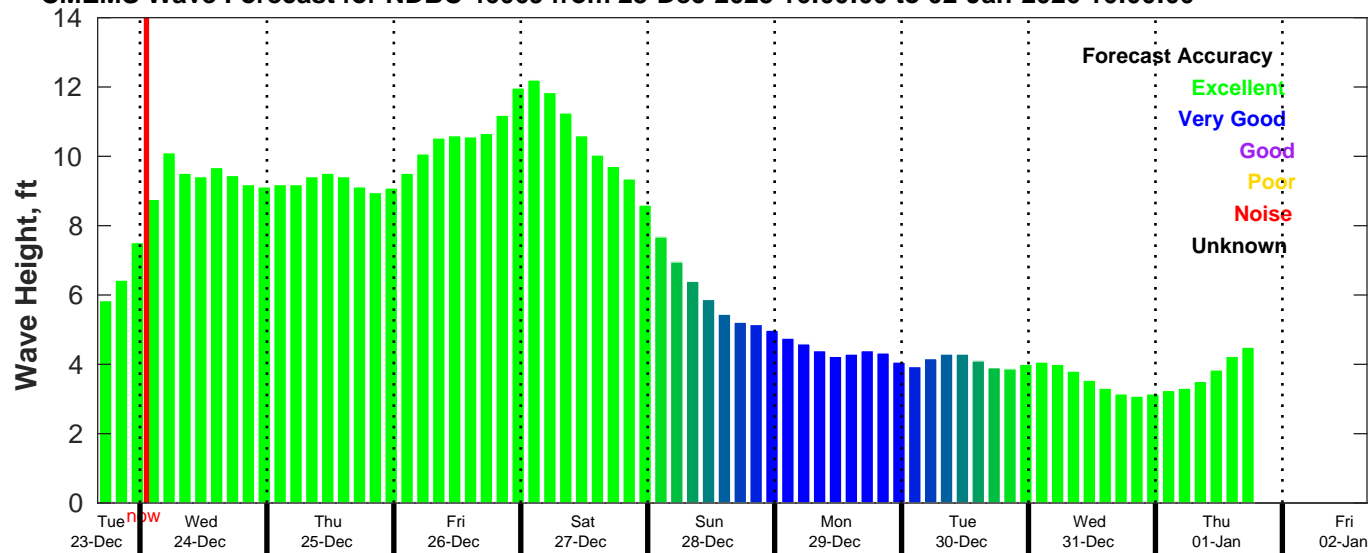
CMEMS Wave Forecast for NDBC 46069 from 23-Dec-2025 16:00:00 to 02-Jan-2026 16:00:00
