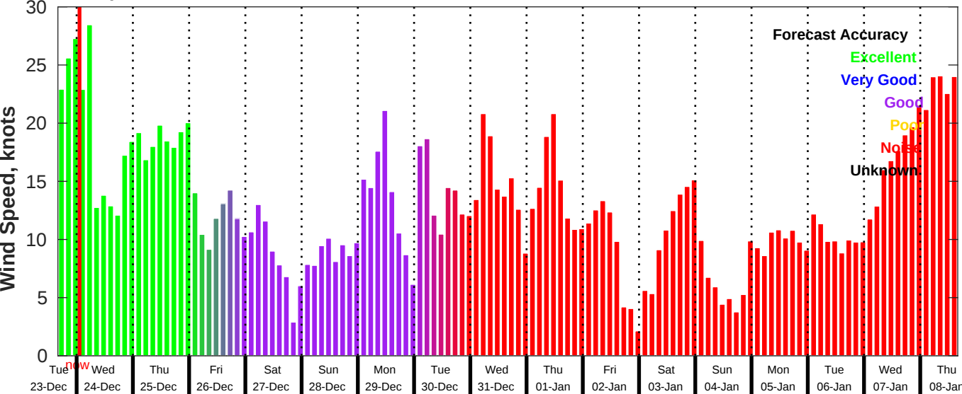
GFS Wind Speed Forecast for NDBC 46069 from 23-Dec-2025 16:00:00 to 08-Jan-2026 16:00:00
