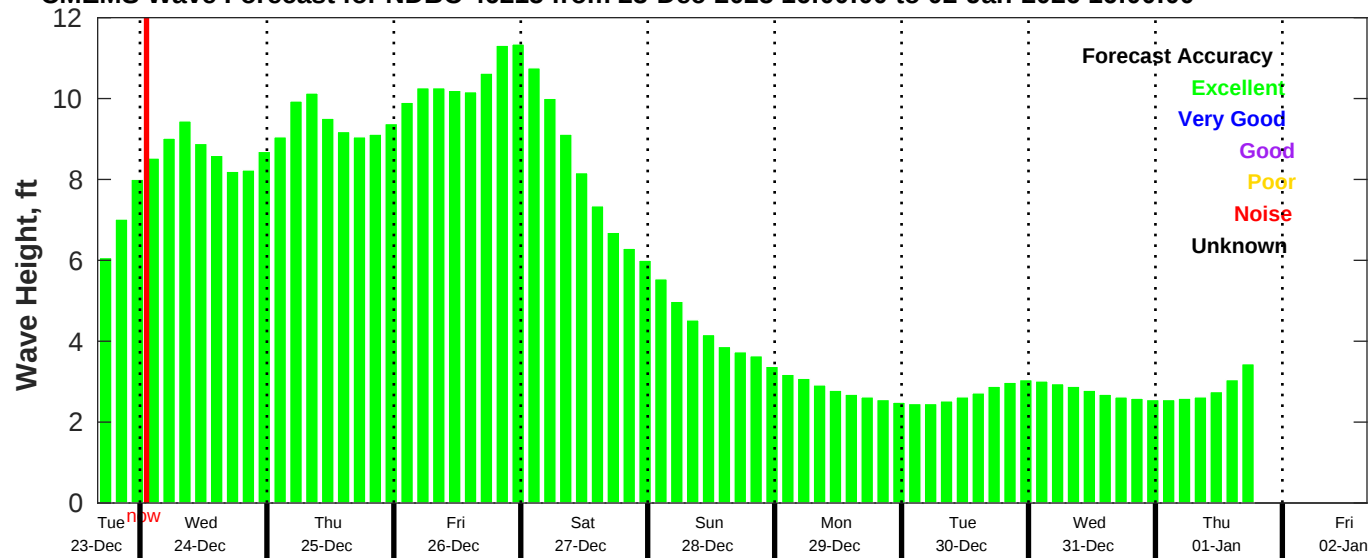
CMEMS Wave Forecast for NDBC 46215 from 23-Dec-2025 16:00:00 to 02-Jan-2026 16:00:00
