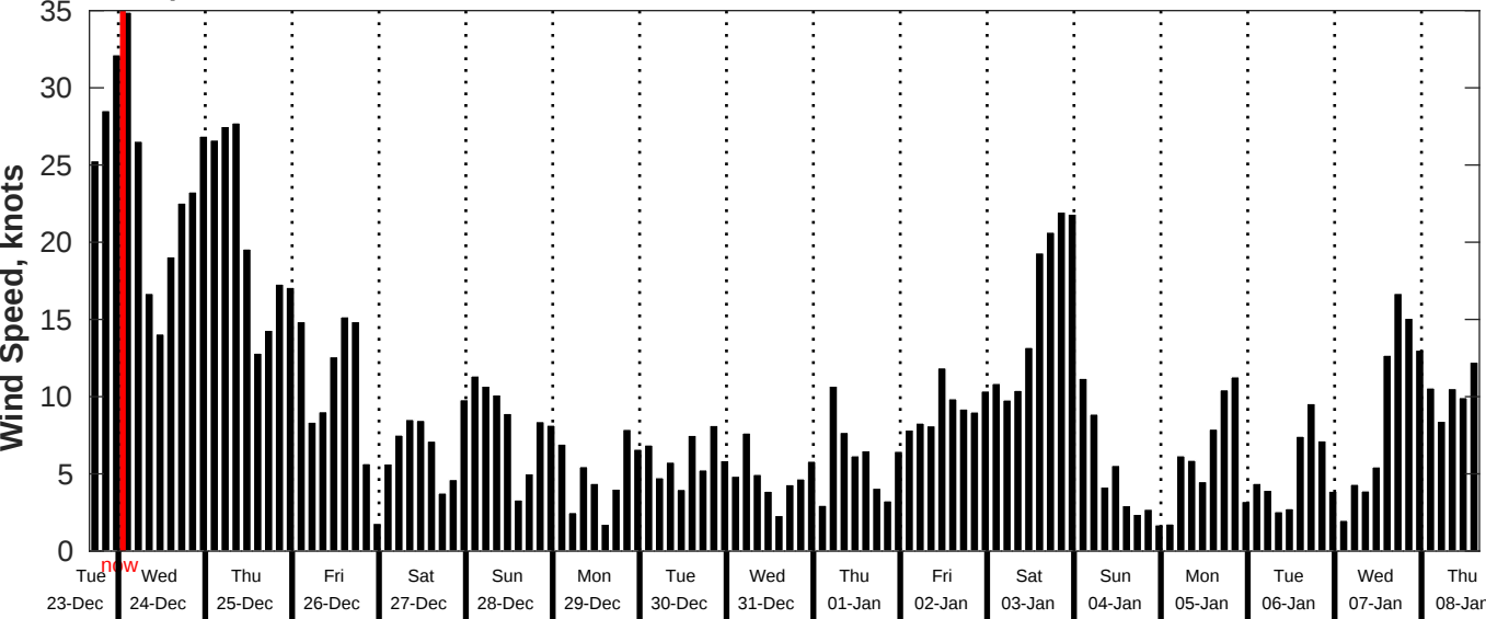
GFS Wind Speed Forecast for NDBC 46215 from 23-Dec-2025 16:00:00 to 08-Jan-2026 16:00:00
