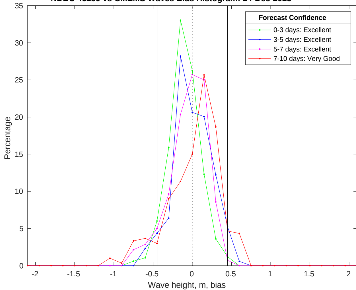
NDBC 46259 vs CMEMS Waves Bias Histogram: 24-Dec-2025
