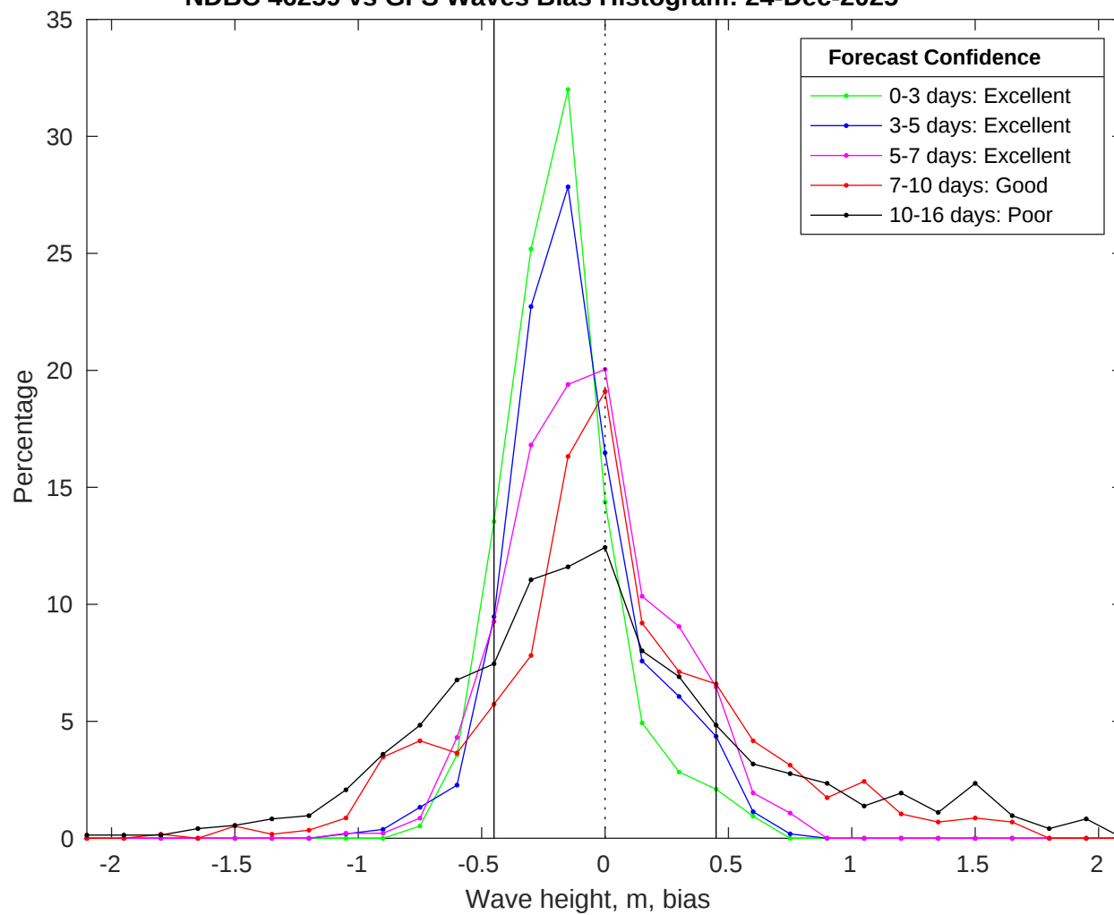
NDBC 46259 vs GFS Waves Bias Histogram: 24-Dec-2025
