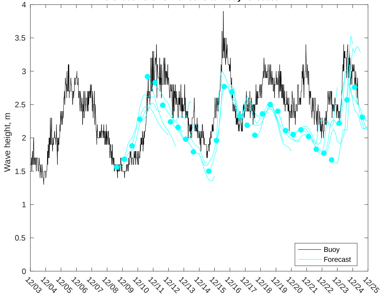
NDBC 51000 vs GFS Waves: 5 to 7 day forecast
