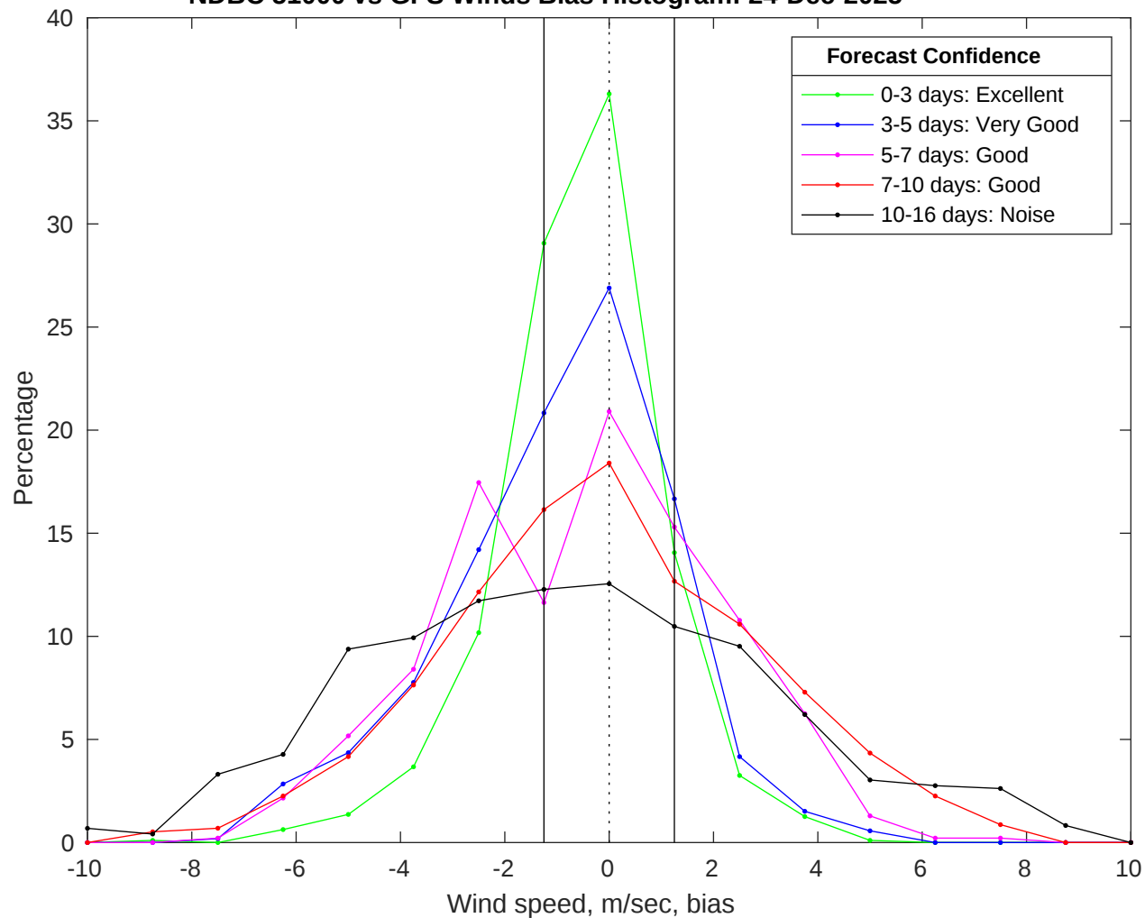
NDBC 51000 vs GFS Winds Bias Histogram: 24-Dec-2025
