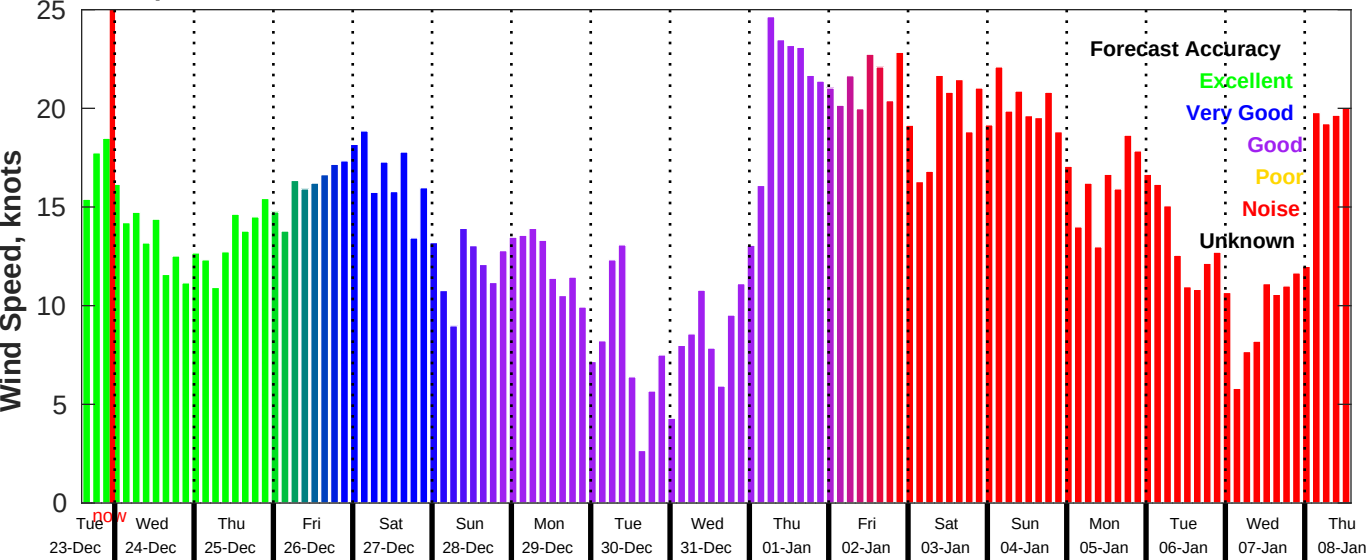
GFS Wind Speed Forecast for NDBC 51000 from 23-Dec-2025 14:00:00 to 08-Jan-2026 14:00:00
