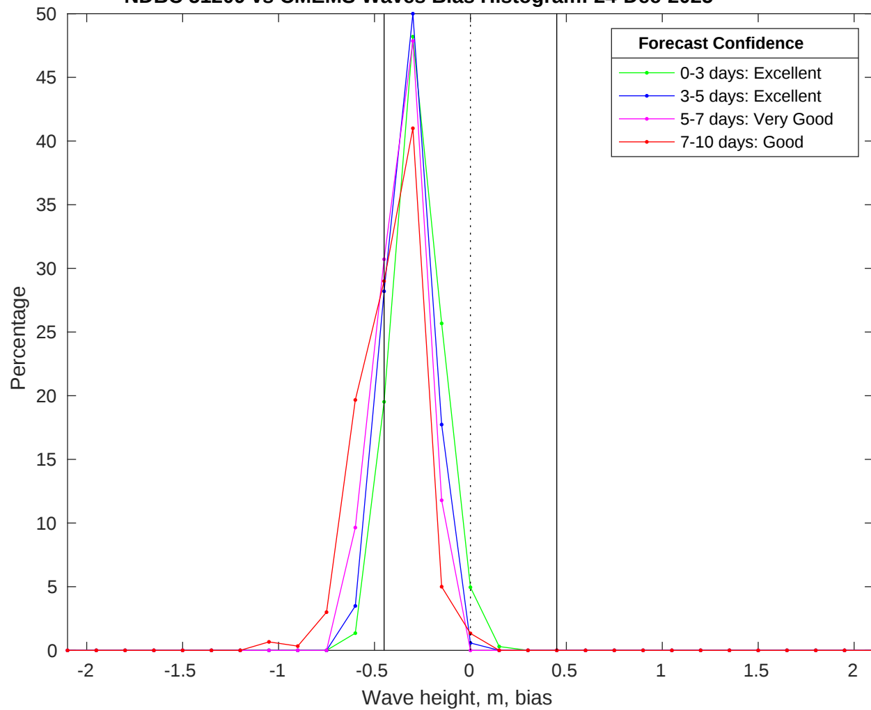
NDBC 51209 vs CMEMS Waves Bias Histogram: 24-Dec-2025
